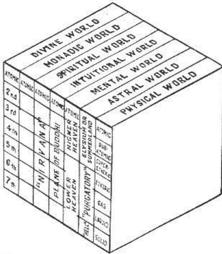
PLANES OF THE SOLAR SYSTEM
